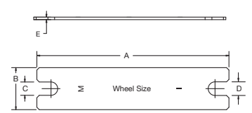
Basic Wheel Plate
