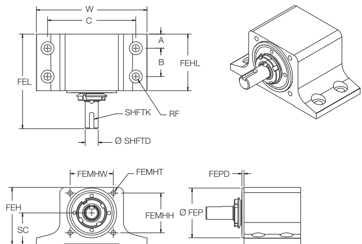
Fixed End
